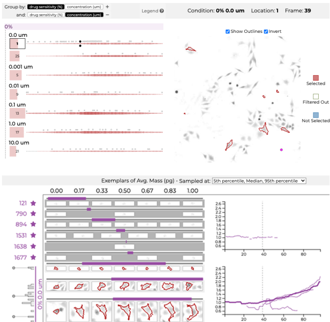
Fig. 11: Loon showing tracking problems in the melanoma dataset. The bookmarked short tracks are in reality a single cell that has not been tracked adequately. This cell would be more accurately represented as a single longer track.
