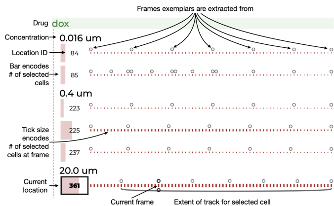
Fig. 5: The image selection view enables analysts to browse images by condition (drug and concentration) and frame. It also displays the number of cells in each frame, and visualizes track lengths for selected cells.
