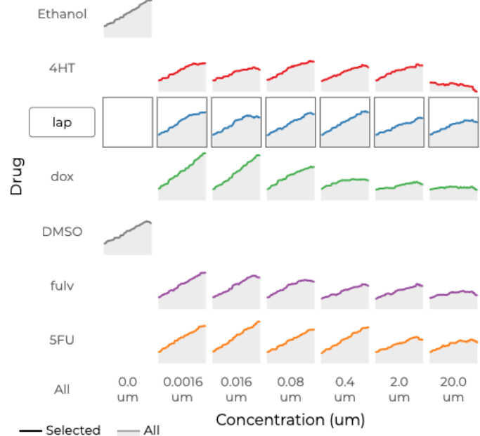
Fig. 3: Condition Selection View. Small area charts show the growth rate for individual conditions. The charts are arranged by drug (4HT, lap, dox, fulv, and 5FU) or control (ethanol and DMSO) type vertically, and by concentration horizontally. Drugs are color coded; controls are shown in gray. Each condition can be selected individually, or conditions can be selected in bulk by row or column.
