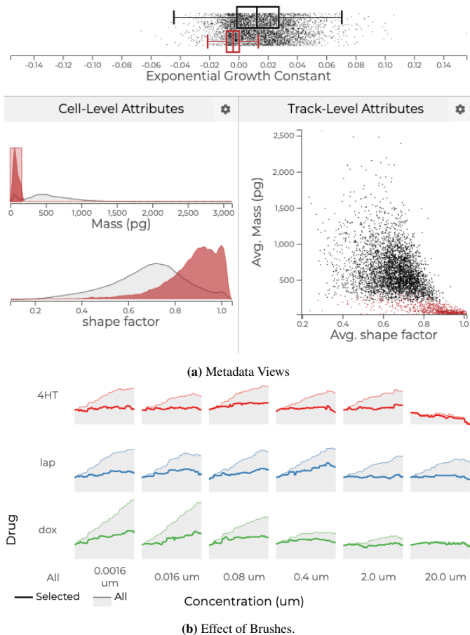
Fig. 10: Metadata views and selections. (a) Histograms, dot plots, and KDE plots visualize metadata. A brush on mass is reflected in all other plots, including in (b) condition selection views’ growth curves. Here, a new growth curve, only for the selected elements, is overlaid.
