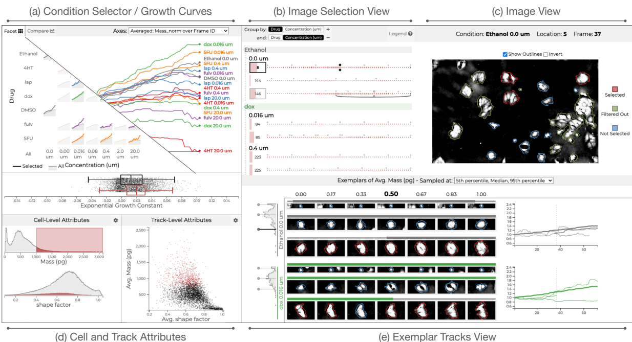
Fig. 1: Overview of the Loon Visualization Tool. (a) The Condition Selector visualizes cell growth rates for different drugs at different concentrations using small multiple line charts in a matrix. Analysts can pick conditions that show interesting behavior for detailed analysis. (b) The Image Selection View is used to navigate images and visualizes aggregate cell and track (cells tracked over time) properties. (c) The Image View shows a selected microscopy image and the segmentation of cells. (d) The Cell and Track Attributes View shows distributions of and correlations between attributes of cells and tracks and serves as the primary means to define selections and filters. (e) The Exemplar Cells View shows cells extracted from the images and samples from a user-specified distribution. It also shows the growth curves for the condition and the selected cells.
