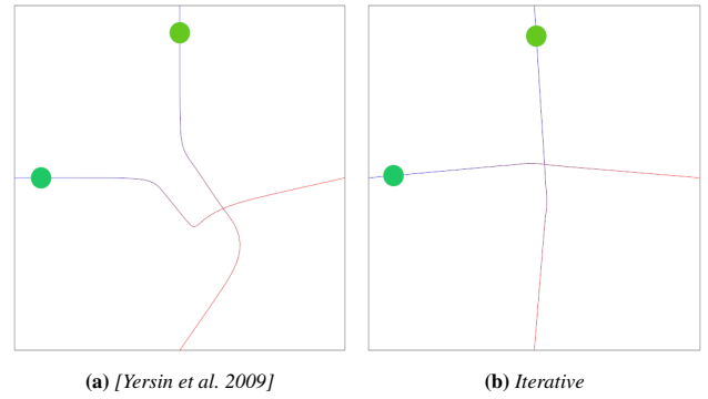
Figure 7: Collision Anticipation (a) Using the approach described in [Yersin et al. 2009] trajectories lack anticipation as they suddenly curve when collisions are near whereas (b) the proposed method generates trajectories with higher anticipation resulting in gradually changing direction.
