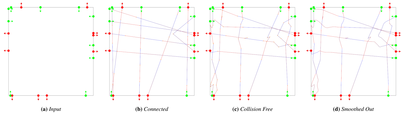
Figure 8: Method example The proposed method starts from (a) a set of control points in the boundaries of an empty patch, (b) interconnects them in an optimal way, (c) resolves any temporal collisions and finally (d) smooths the trajectories.
